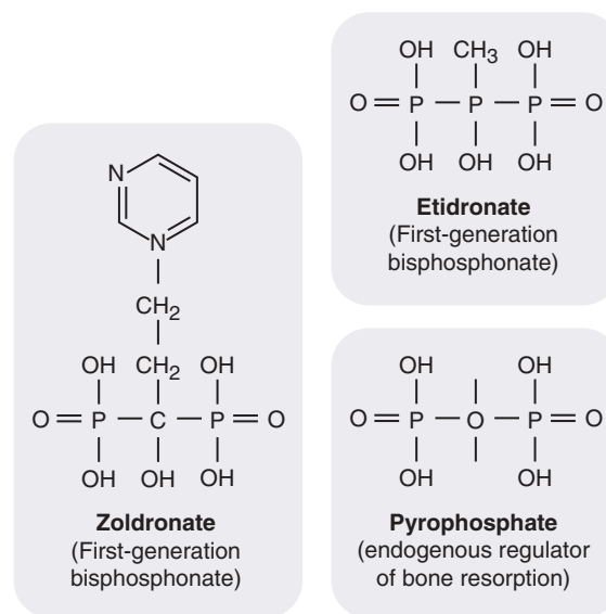
Fig. 35.5 Structure of bisphosphonates. Replacement of the oxygen atom in pyrophosphate renders the compounds enzyme resistant. Addition of an N-containing side chain alters the mechanism of action (see text) and greatly increases potency.
