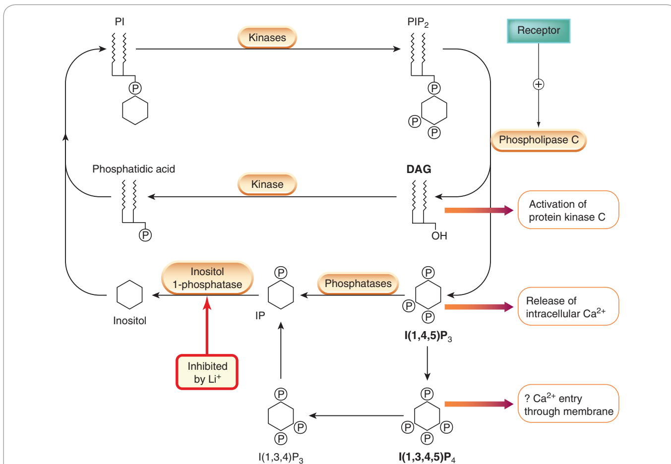
Fig. 3.12 The phosphatidylinositol (PI) cycle. Receptor-mediated activation of phospholipase C results in the cleavage of phosphatidylinositol bisphosphate (PIP 2 ), forming diacylglycerol (DAG) (which activates protein kinase C) and inositol trisphosphate (IP 3 ) (which releases intracellular Ca 2+ ). The role of inositol tetraphosphate (IP 4 ), which is formed from IP 3 and other inositol phosphates, is unclear, but it may facilitate Ca 2+ entry through the plasma membrane. IP 3 is inactivated by dephosphorylation to inositol. DAG is converted to phosphatidic acid, and these two products are used to regenerate PI and PIP 2 .
