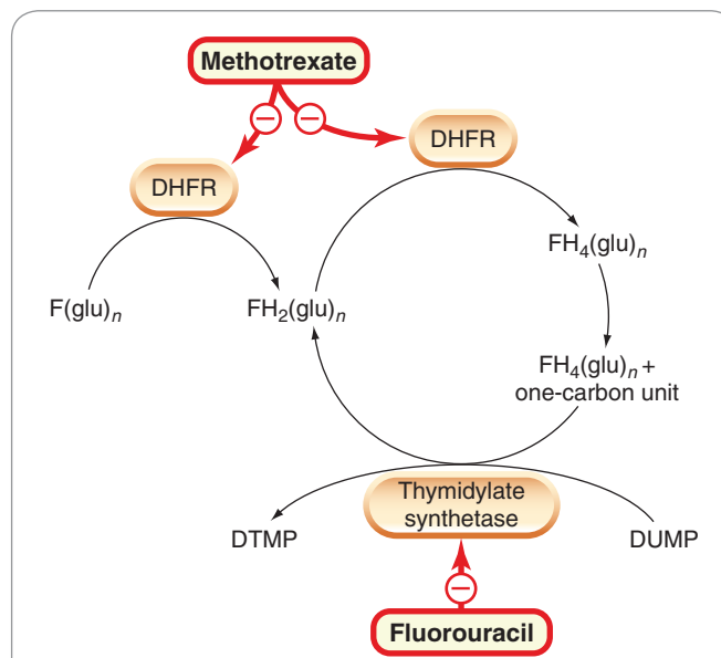
Fig. 55.6 Simplified diagram of action of methotrexate and fluorouracil on thymidylate synthesis. Tetrahydrofolate polyglutamate \text{FH}_4(\text{glu})_n functions as a carrier of a one-carbon unit, providing the methyl group necessary for the conversion of 2'-deoxyuridylylate (DUMP) to 2'-deoxythymidylylate (DTMP) by thymidylate synthetase. This one-carbon transfer results in the oxidation of \text{FH}_4(\text{glu})_n to \text{FH}_2(\text{glu})_n . Fluorouracil is converted to FDUMP, which inhibits thymidylate synthetase. DHFR, dihydrofolate reductase.
