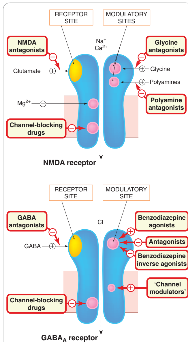
Fig. 37.5 Main sites of drug action on NMDA and \text{GABA}_A receptors. Both receptors are multimeric ligand-gated ion channels. Drugs can act as agonists or antagonists at the neurotransmitter receptor site or at modulatory sites associated with the receptor. They can also act to block the ion channel at one or more distinct sites. In the case of the \text{GABA}_A receptor, the mechanism by which 'channel modulators' (e.g. ethanol, anaesthetic agents) facilitate channel opening is uncertain; they may affect both ligand binding and channel sites. The location of the different binding sites shown in the figure is largely imaginary, although study of mutated receptors is beginning to reveal where they actually reside. Examples of the different drug classes are given in Tables 37.1 and 37.3.
